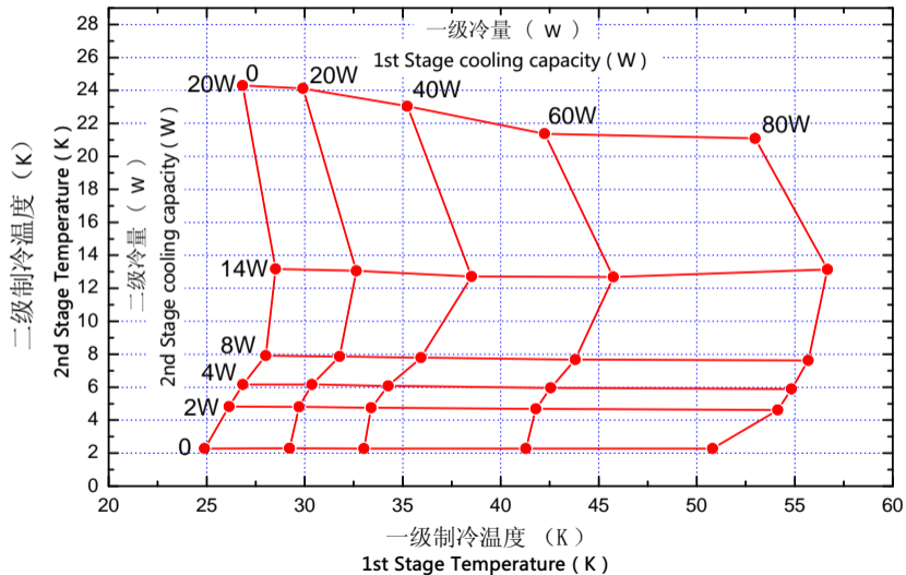
KDE410 制冷量典型曲线图 (50Hz) KDE410 Typical Load Map ( 50Hz )
